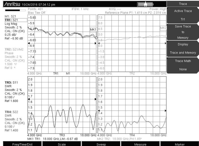
Amplitude, Phase Input and Output Return Losses
