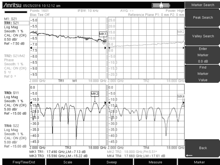
Amplitude, Phase Input and Output Return Losses
